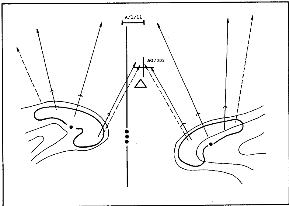
Figure 45.--Coverage for a Gap.
