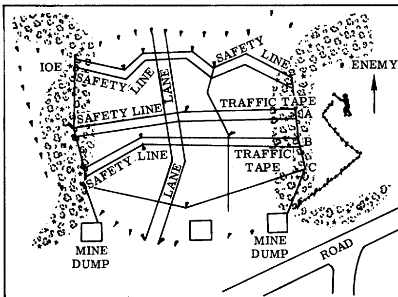
Figure 79.--Minefield Layout by Tape.
