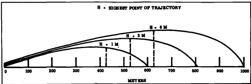
Figure 2-3. Diagram Showing Maximum Ordinate (H) of Trajectory.
