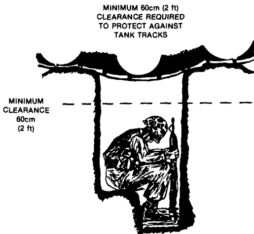
Figure 5-14. One-Man Fighting Hole Protects Against Tanks.
