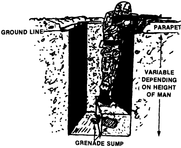
Figure 5-12. One-Man Fighting Hole. (Horizontal View)
