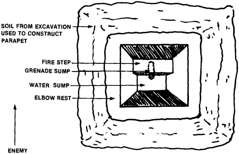
Figure 5-12. One-Man Fighting Hole. (Horizontal View)
